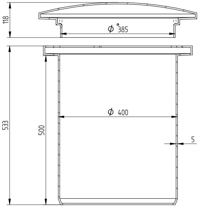
SECTION F-F
