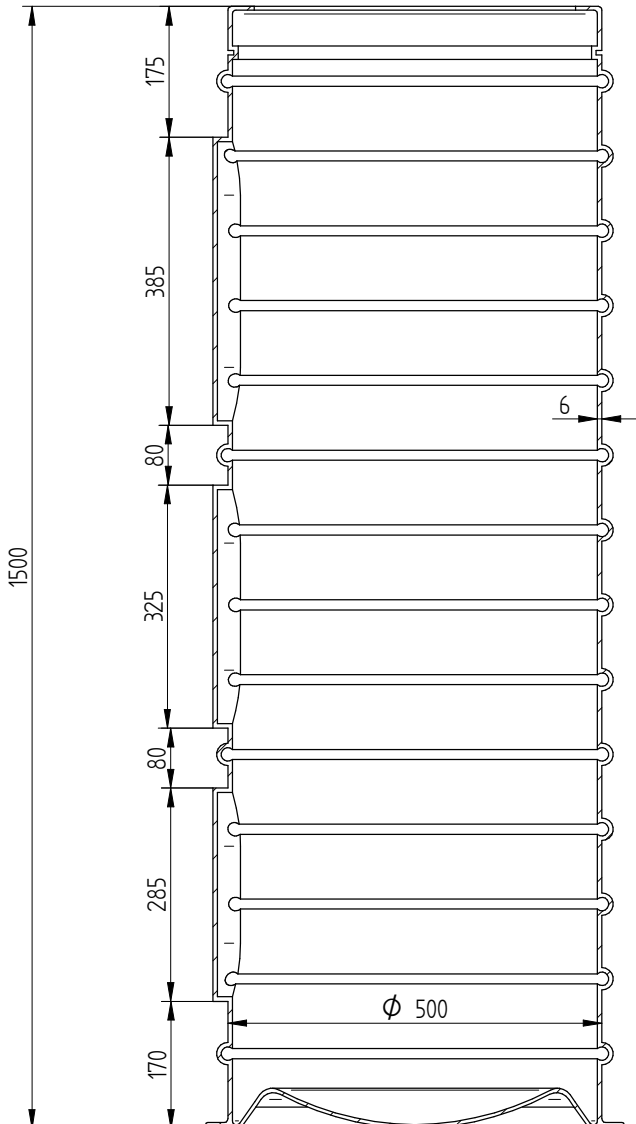
SECTION C-C
